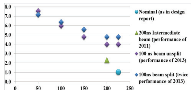
Figure 1: Expected peak luminosity ( 10^{27} Hz/cm 2 ) at 7 ZTeV, with respect to batch spacing in the SPS (ns).
