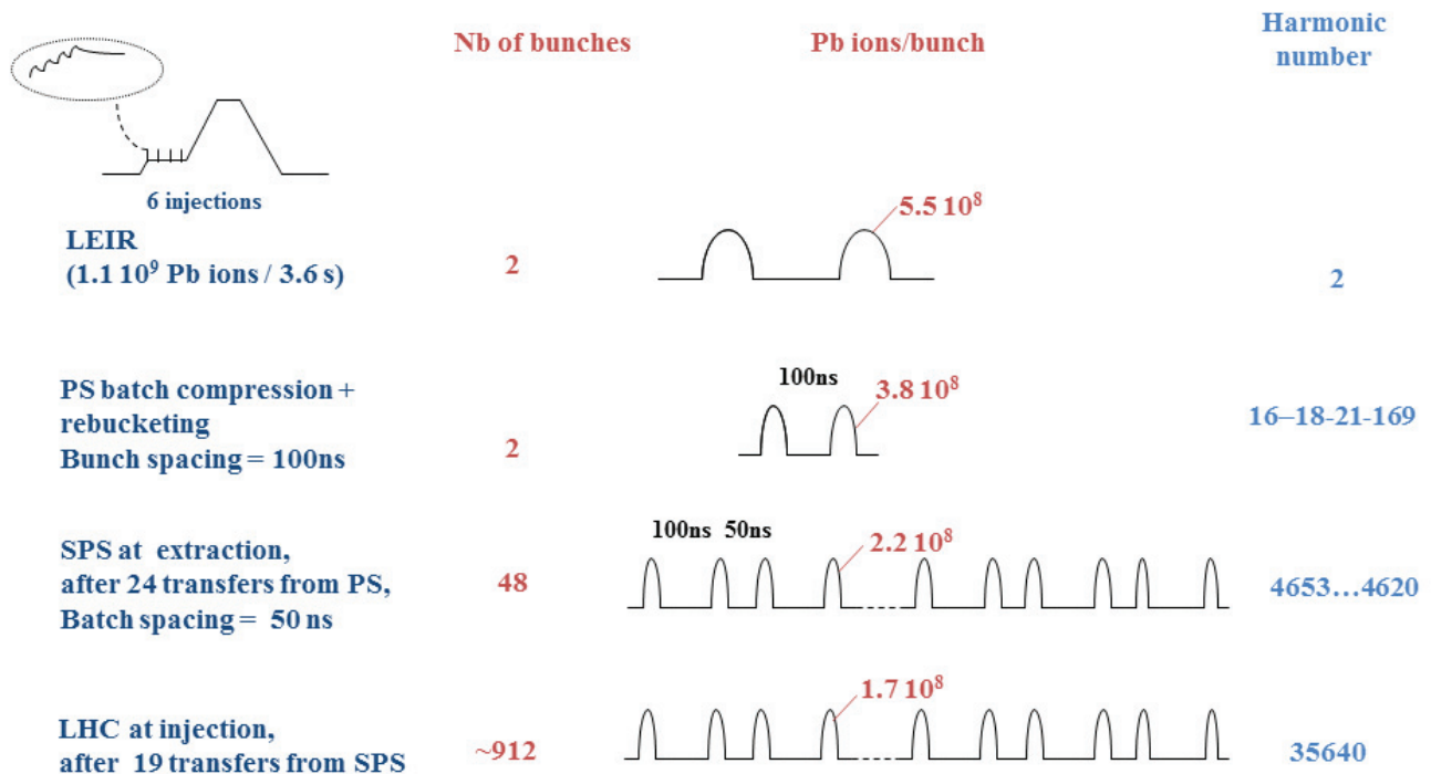
Figure 2: Alternating 100/50 ns spacing scheme, with 24 PS injections into the SPS. The beam intensities correspond to the ones achieved for the p-Pb run in 2013.
