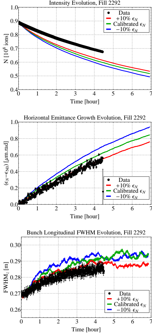
Figure 4: Evolution of a single bunch compared to simulation. Top: intensity, middle: emittance, bottom: longitudinal FWHM.
