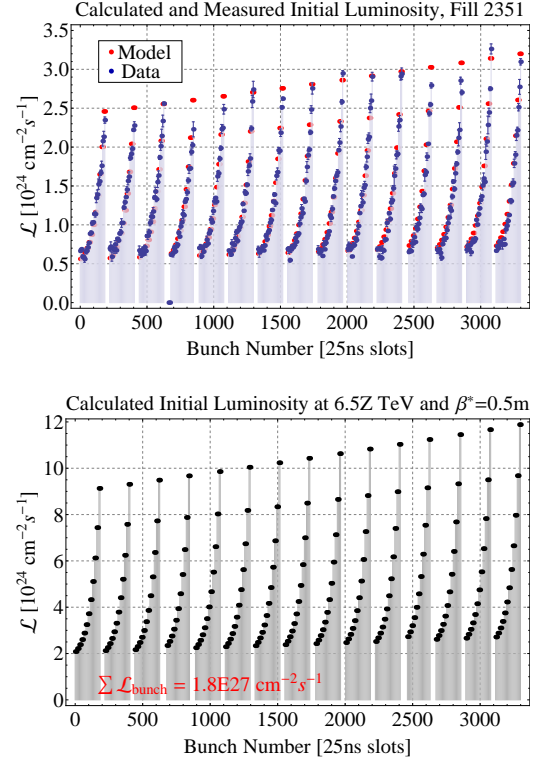
Figure 5: Bunch-by-bunch model ( E = 3.5Z TeV, top) and estimate ( E = 6.5 TeV bottom) of the initial luminosity.
