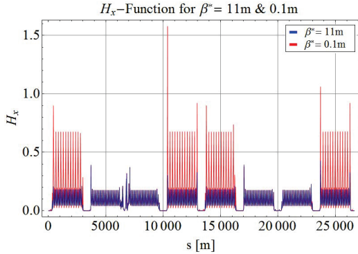
Figure 2: Horizontal \mathcal{H} -function.
