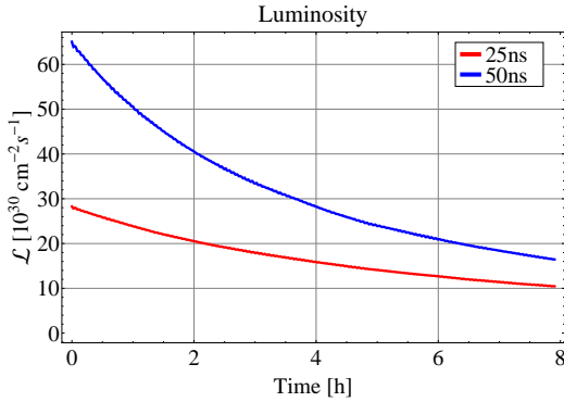
Figure 5: Simulated single bunch luminosity evolution per bunch crossing (without levelling and crab-cavities).
