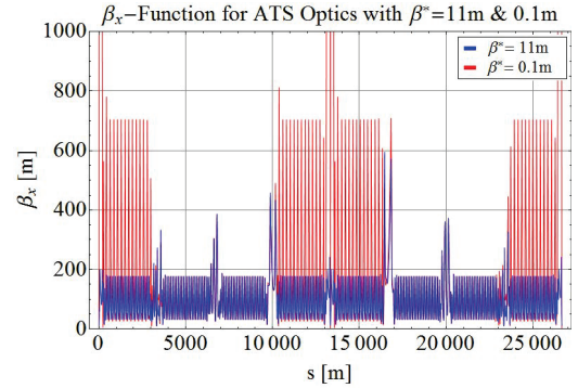
Figure 1: \beta -functions for ATS optics with \beta^* = 11 m (blue) and 0.1 m (red) in IP 1 and 5.
