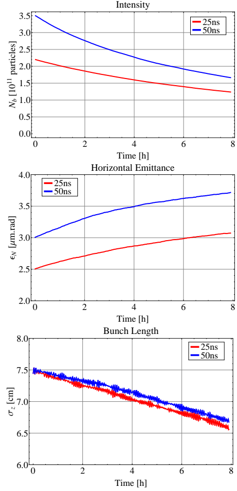
Figure 6: Simulated bunch evolution.
