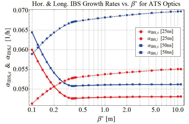
Figure 4: IBS growth rates along the squeeze.
