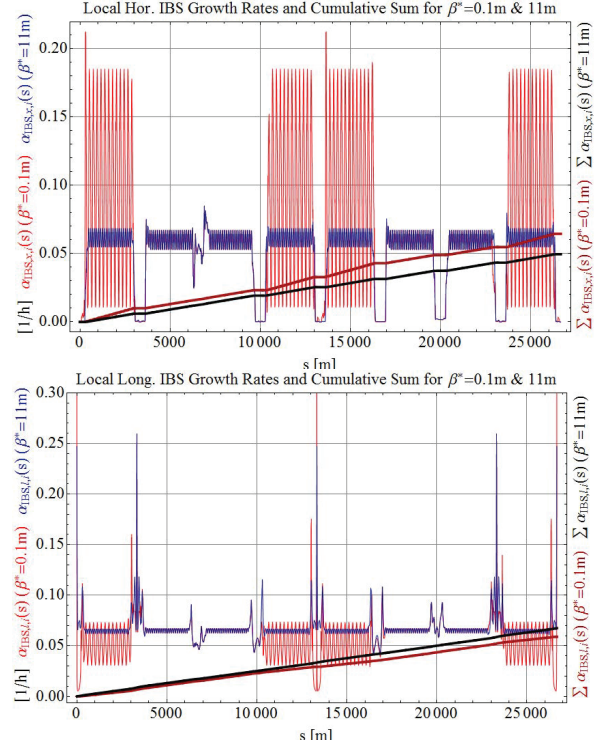
Figure 3: Local contribution of the IBS growth rates. Top: horizontal, bottom: longitudinal plane.
